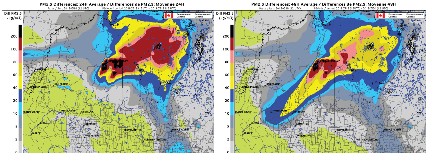
Figure 10: Examples of the FireWork products prepared for the May 2016 Fort McMurray wildfire event in northern Alberta, showing the forecasted wildfire emissions contribution to surface PM 2.5 concentrations (µg/m 3 ) over a 24-hour period (left) and a 48-hour period (right). These examples were both produced by the 2016-05-18 12 UTC run.
