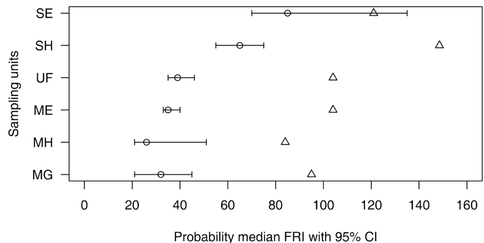
Figure 2 Median FRI since the onset of effective fire suppression (triangle) in comparison to the natural range of variation depicted by the 95% lower and upper confidence intervals of the Kaplan-Meier probability median fire interval. ME: Montane-East, MG: Montane-Ghost, MH: Montane-Highwood, SE: Subalpine-Elbow, SH: Subalpine-Highwood, UF: Upper Foothills.
