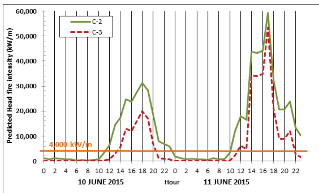
Figure 7. Headfire Intensity curves for C-2 and C-3 fuel types on 10 and 11 June 2015 using hourly weather data from E5. The diurnal (Lawson) method was used to adjust hourly FFMFC.
