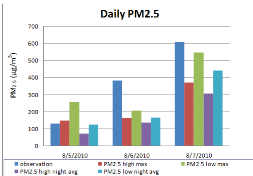
Figure 11: Comparison of PM_{2.5} concentrations calculated with two different plume heights to observations (in dark blue) in Moscow. Red indicates the daily maximum modelled with WRF’s boundary layer heights (“high”) and green corresponds to daily maximum when plumes stay below 600 m (“low”). Nighttime averages are shown in purple for high plume injection and in light blue for lower injection.
