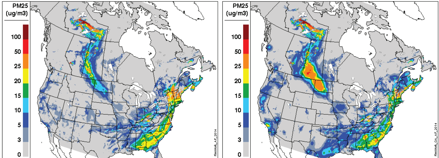
Figure 8: PM 2.5 surface concentrations on 9 July 2014 forecasted by FireWork (left) and adjusted by RDAQA FW (right).
