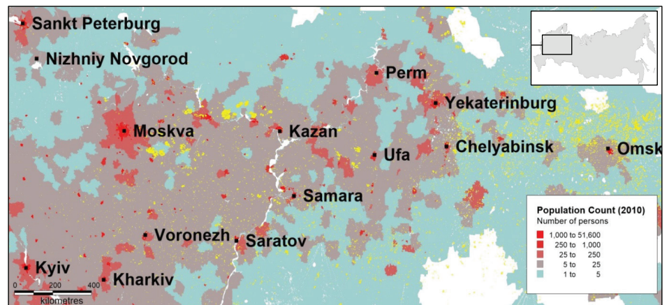
Figure 1. Area burned (in yellow) by forest and peat fires in western Russia in 2010. Population count is given as the number of persons/grid cell (30 arc second ~1km) [Center for International Earth Science Information Network - CIESIN - Columbia University, 2016]. Moscow is the most populous city of the Russian Federation with nearly 17 million residents within its urban area.
