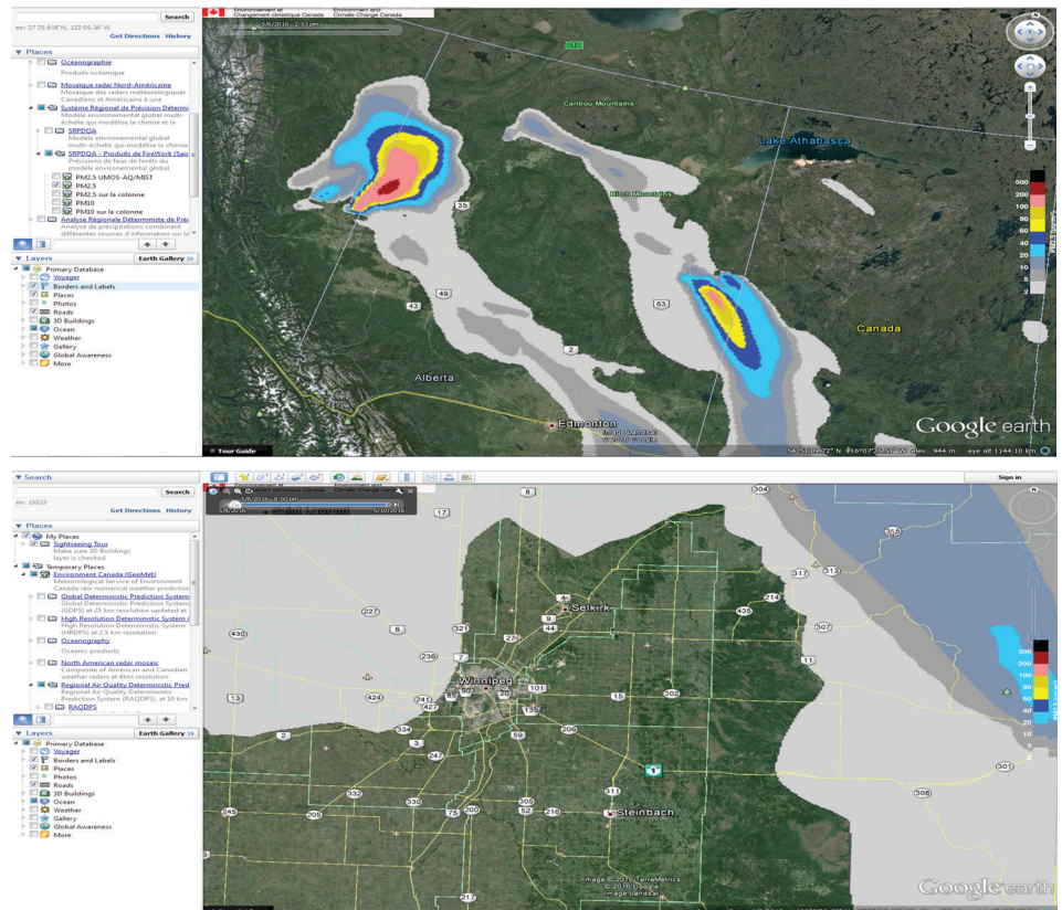
Figure 5: Forecasted wildfire emissions contribution to surface PM_{2.5} concentrations ( \mu g/m^3 ) valid at 2016-05-06 12UTC as forecasted by the 2016-05-06 00UTC FireWork run (upper image), and a close-up of the surface PM_{2.5} concentration field two days later over southern Manitoba valid at 2016-05-08 20UTC as forecasted by the 2016-05-08 00UTC run (lower image). These examples were produced using ECCC Geospatial Web Services and displayed using the Google Earth™ program.
