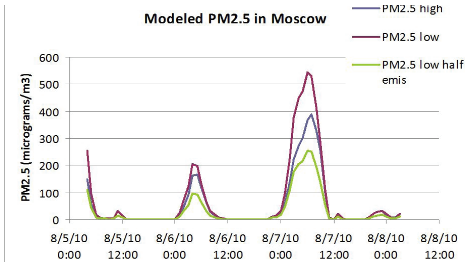
Figure 10: Hourly variation of PM_{2.5} concentrations calculated at the Moscow location with three CMAQ runs using different emission scenarios. The blue color represents the concentrations calculated with the plume heights (primarily above the boundary layer) and emissions predicted with the modeling system; red denotes concentrations simulated with the predicted emissions, but injected closer to the surface (in the boundary layer); and green corresponds to half of the predicted emissions and injected closer to the ground.
