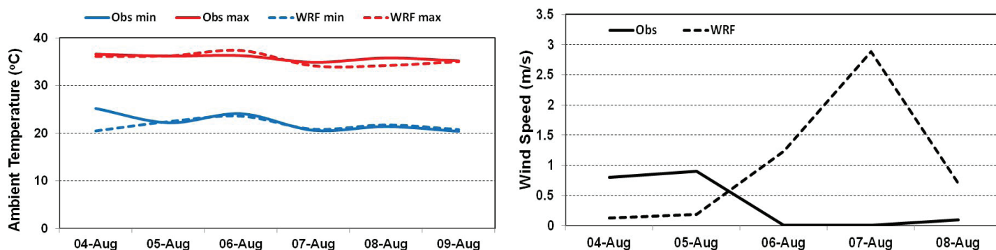
Figure 8: Comparison of surface (a) air temperatures and (b) wind speed observed and simulated with WRF at Moscow during early August 2010.
