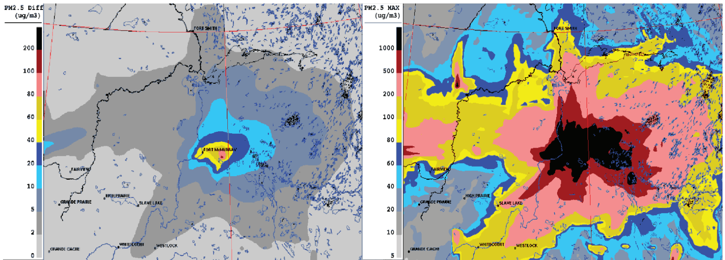
Figure 11: Forecasted wildfire emissions contribution to mean monthly PM_{2.5} concentrations at the surface (left) and to maximum hourly PM_{2.5} concentrations ( \mu g/m^3 ) forecasted by FireWork (right) for May 2016.
