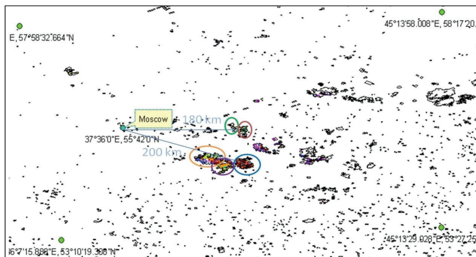
Figure 6: Location of the five major wildland fires whose smoke plumes affected Moscow's air quality during the first week of August 2010. The geographical boundaries of the CMAQ simulation domain are indicated by the four green dots.
