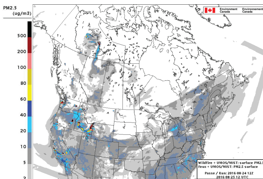
Figure 7: Examples of the post-processed UMOS-AQ/MIST PM_{2.5} concentration field ( \mu g/m^3 ) based on by 2016-08-24 12UTC FireWork run and valid at 2016-08-25 12UTC.
