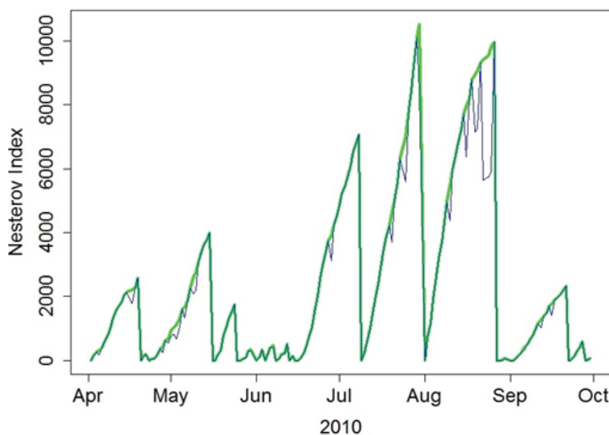
Figure 3: Nesterov Index (in green) and Modified Nesterov Index (in blue) from April through September 2010 in the region of Moscow (55°45'N, 37°37'E). Four fire danger classes are usually considered based on NI or MNI values: minimal (0-300), moderate (301-1000), high (1001-4000) and extreme (4001+).
