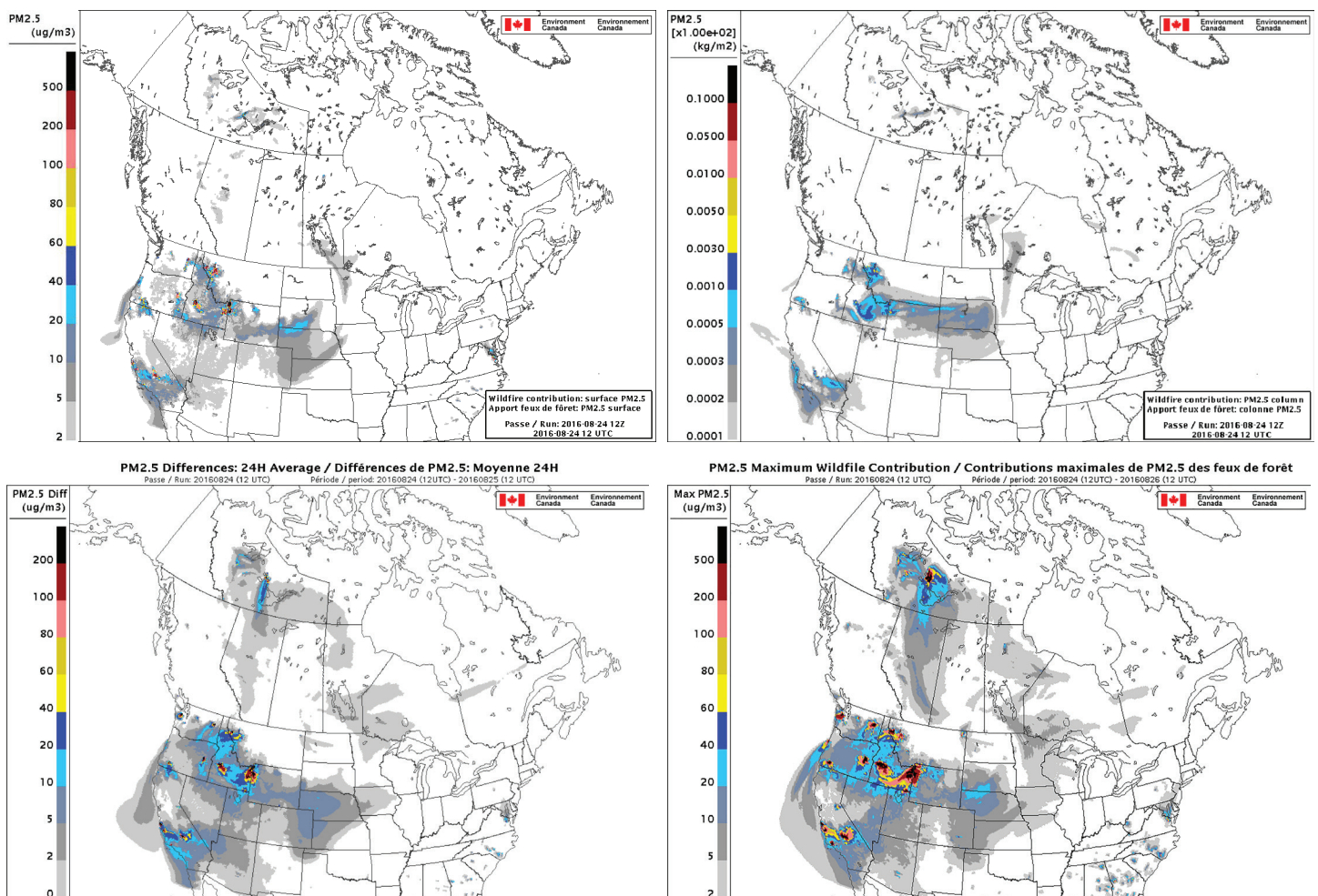
Figure 6: Examples of FireWork forecasts of wildfire emissions contributions to PM 2.5 concentrations (ug/m 3 ) at surface level (upper-left panel), for total column (upper-right panel), averaged over 24 hours (lower-left panel), and maximum hourly values over 24 hours (lower-right panel). These examples are forecasted by the 2016-08-24 12UTC run.
