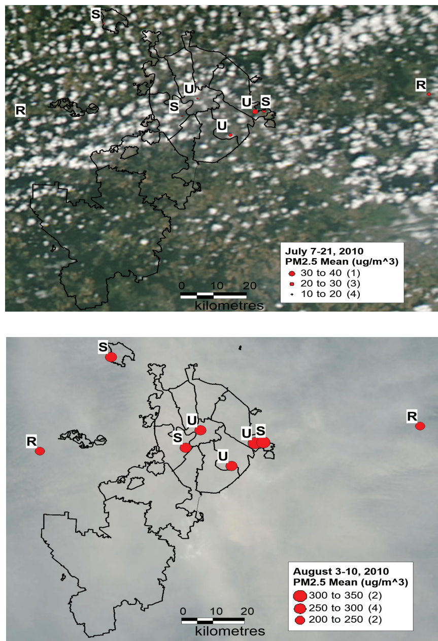
Figure 5: PM_{2.5} concentrations measured in the Moscow region before (top) and during (bottom) the smoke event of 2010. Polygons represent the twelve administrative divisions (“okrugs”) of the Russian capital ( http://gis-lab.info/qa/moscow-atd.html , accessed 10 September 2016). The eight ambient air quality monitoring stations are classified as follows: urban (U), suburban (S) or rural background (R). MODIS Aqua scenes (250 m resolution) of the Moscow region show cloudy conditions on July 21st (top) and heavy smoke on August 7th (images courtesy of NOAA/NASA).
