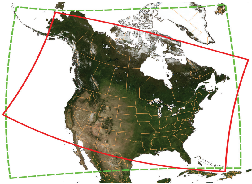
Figure 1: FireWork domain boundaries prior to (red) and post (green) September 7th 2016.
