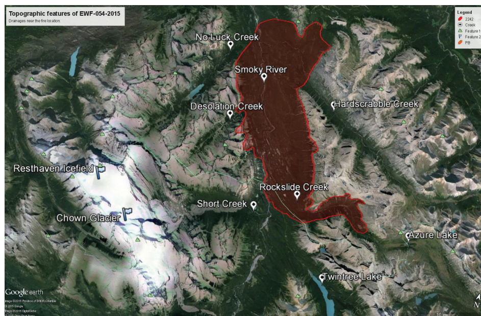
Figure 3. Main valleys and drainages near the Rockslide Creek wildfire.
