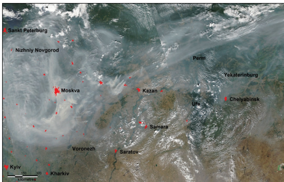
Figure 4: MODIS image of smoke plumes over Western Russia, 7 August, 2010 (image courtesy of NOAA/NASA). Red polygons correspond to areas with population count of 1000+/km 2 [Center for International Earth Science Information Network - CIESIN - Columbia University, 2016].
