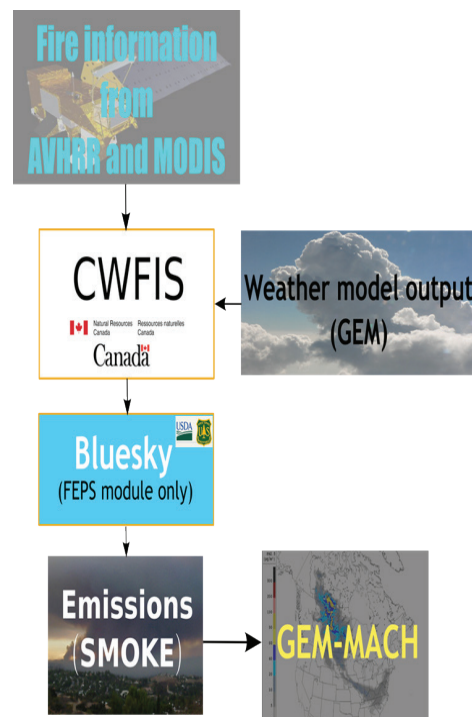
Figure 3: FireWork model system framework and data flow
