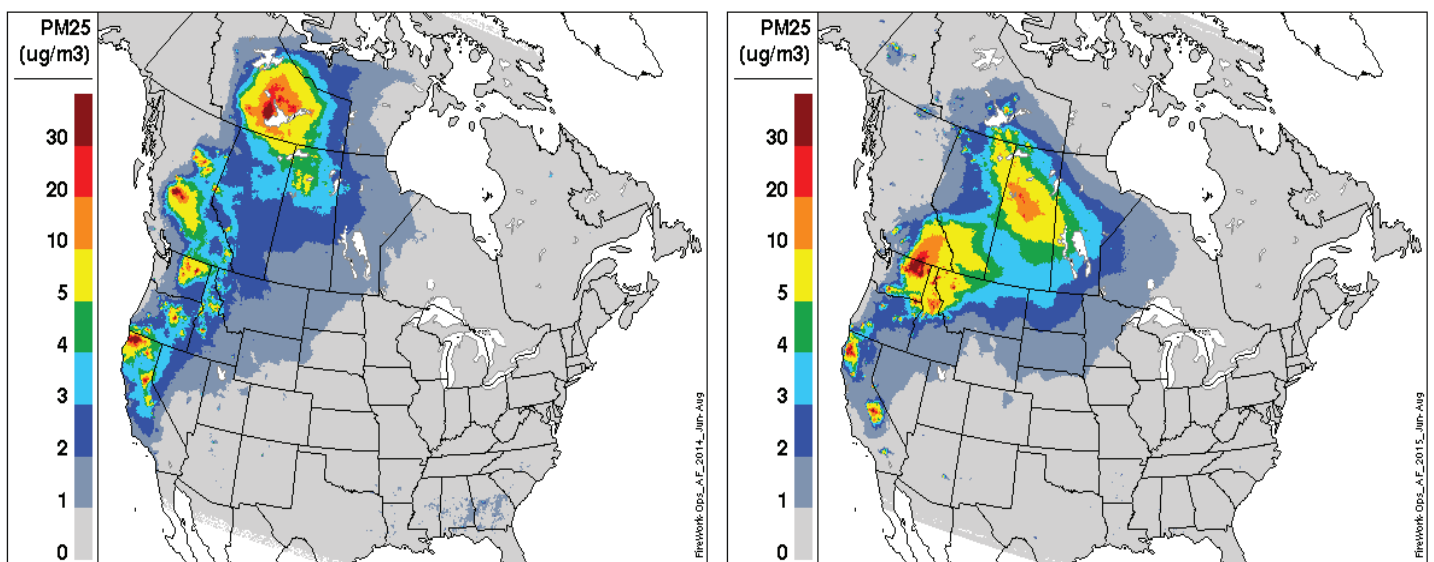
Figure 2: Forecasted summertime (June-August) 2014 (left) and 2015 (right) wildfire emissions contribution to 3-month average one-hour surface PM_{2.5} concentrations ( \mu g/m^3 ).
