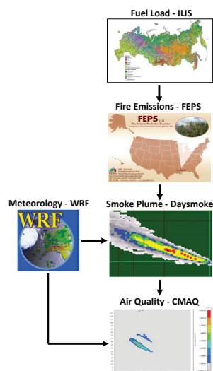
Figure 7: Overview of the five components of the wildland fire & smoke modeling system applied to the 2010 Russian fires.
