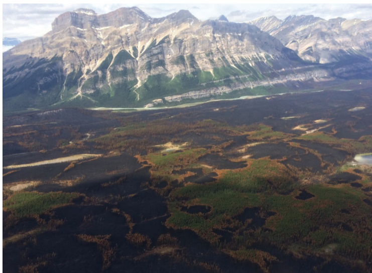
Figure 5. Evidence of short range spotting on Rockslide Creek wildfire looking west perpendicular to the Smoky river (Photo: K.Gibos).
