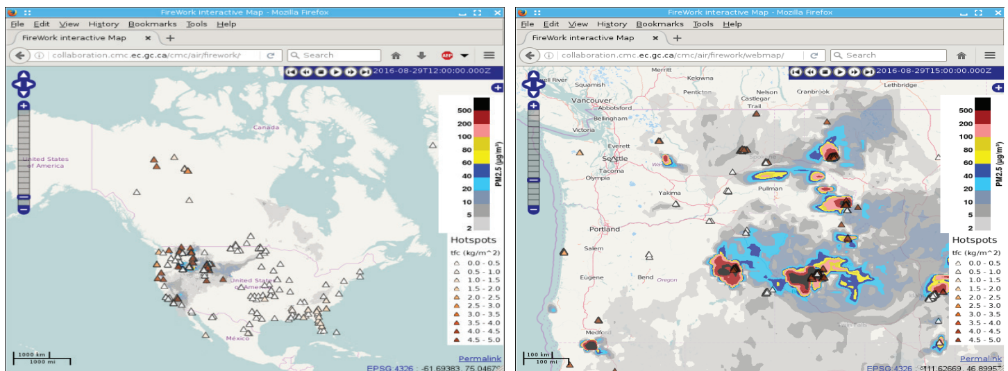
Figure 9: Examples of the interactive FireWork webmaps over the FireWork domain (left) and zoomed over the western U.S. and Canada (right) showing Total Fuel Consumption (TFC) values representing flaming combustion (kg/m 2 ), and the contribution of forecasted wildfire emissions to PM 2.5 surface concentrations (µg/m 3 ), valid at 2016-08-29 12UTC (left) and 15UTC (right) from the 2016-08-29 12UTC FireWork run.
