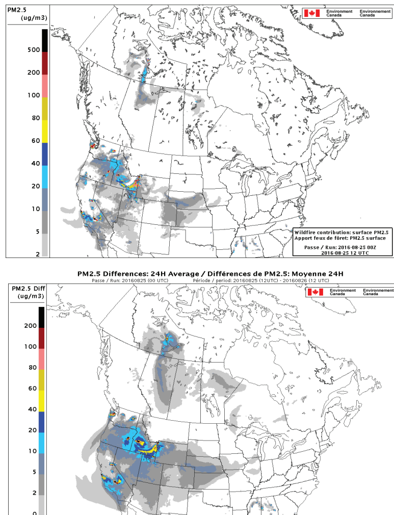
Figure 4: Forecasted wildfire emissions contribution to surface PM 2.5 concentrations (µg/m 3 ) valid at 2016-08-25 12UTC (top) and averaged over 24 hours (2016-08-25 12UTC to 2016-08-26 12UTC) (bottom) forecasted by 2016-08-25 00UTC run.
