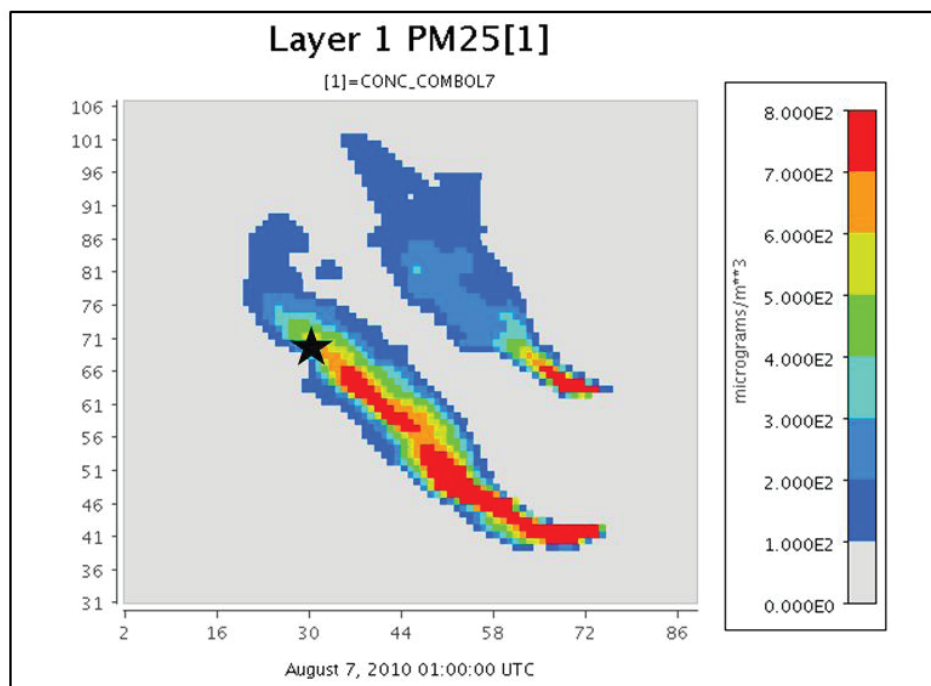
Figure 9: Modelled surface PM 2.5 concentrations on August 7th at 5:00 am local time (1:00 GMT). The location of Moscow is indicated with the black star.
